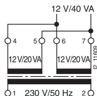
4AC3 140 Parallel switching
