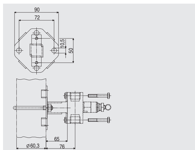
Fig. 1/114 Mounting bracket for wall, rack or pipe mounting, dimensions for 7MF9011-4EA and -4DA, dimensions
